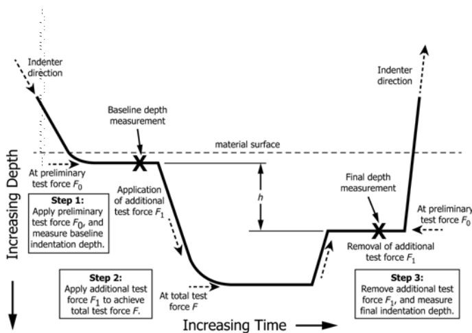
FIG. 1 Rockwell Hardness Test Method (Schematic Diagram)
